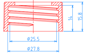
(28/410) CAP, P=1"x6 TPI
